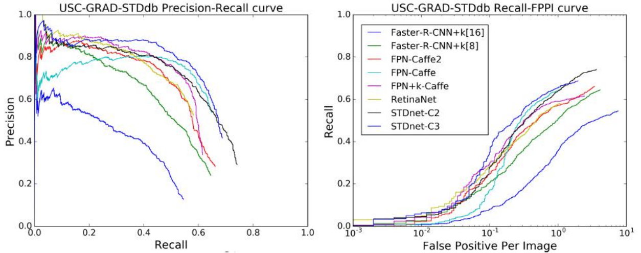
Figure 8: Precision-recall (left) and recall-FPPI (right) curves. The numbers inside the brackets indicate the global effective stride (GES).
